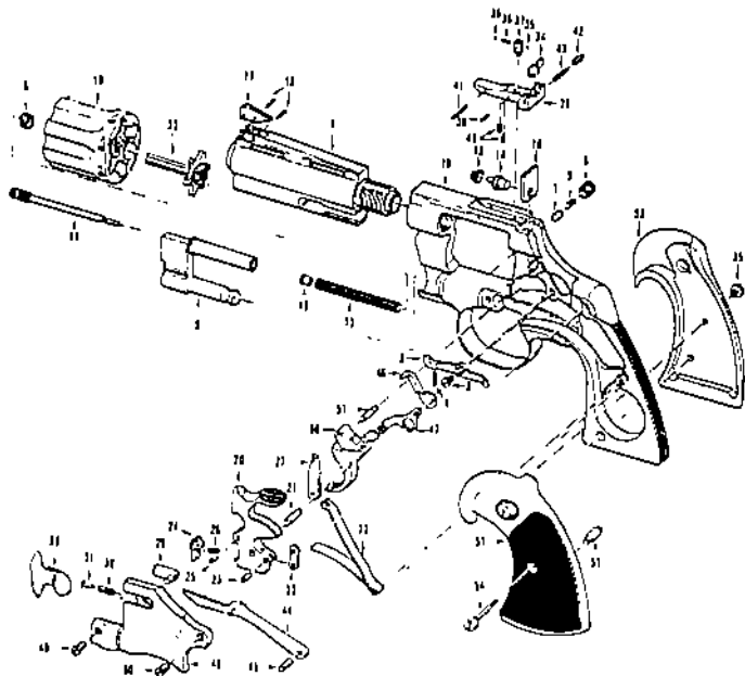
FIGURE 8— PARTS ILLUSTRATION OF PYTHON
